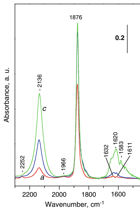
Fig. 4 FTIR spectra (nitrosyl stretching region) of NO adsorbed at 298\text{ K} on Fe-H-BEA zeolite: (a) introduction of a small dose of NO to the sample, (b) in the presence of 940\text{ Pa} NO and (c) after 1\text{ h} . The spectra are background corrected
